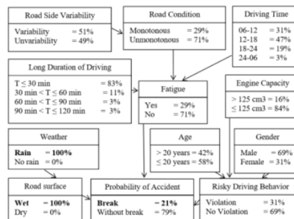
Figure 4. Scenario 2: Effect weather to probability of accident
