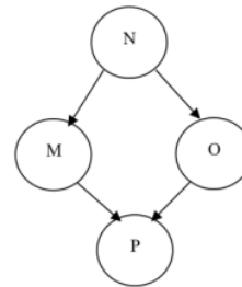
Figure 1. Example of analysis of bayesian network
