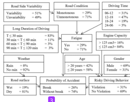
Figure 2. Model Structure bayesian network of probability of accident severity
