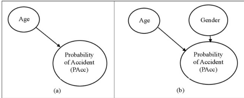
Figure 1. Examples Bayesian Network
