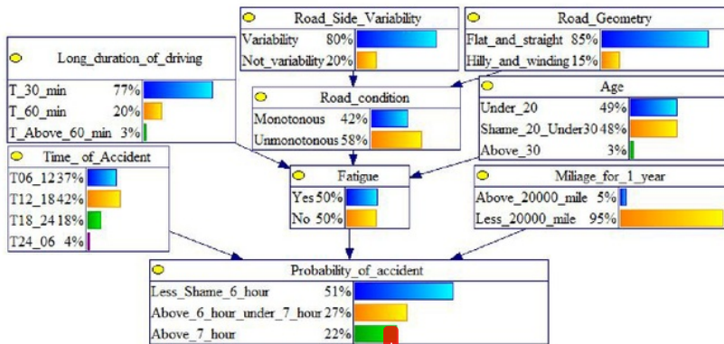
Figure 2. Structure of bayesian network
