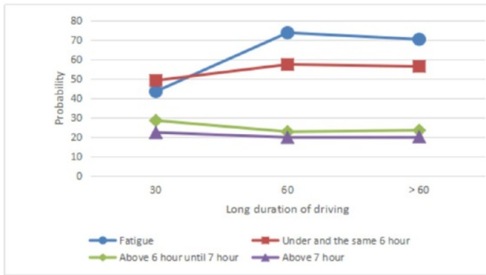
Figure 6. Correlation between long duration of driving with the probability of accident and probability of fatigue
